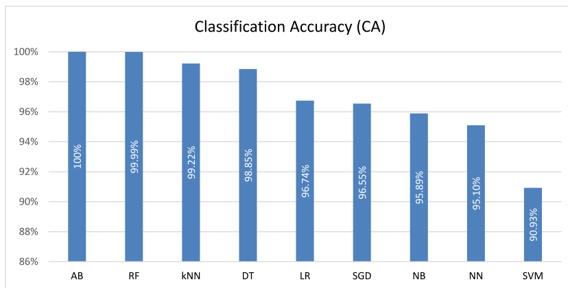
Fig. 4. Average CA scores of all classifiers for recognizing five ADLs.
